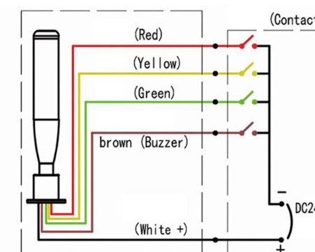
DC24V NPN(Common+)(Constant brightness type)
